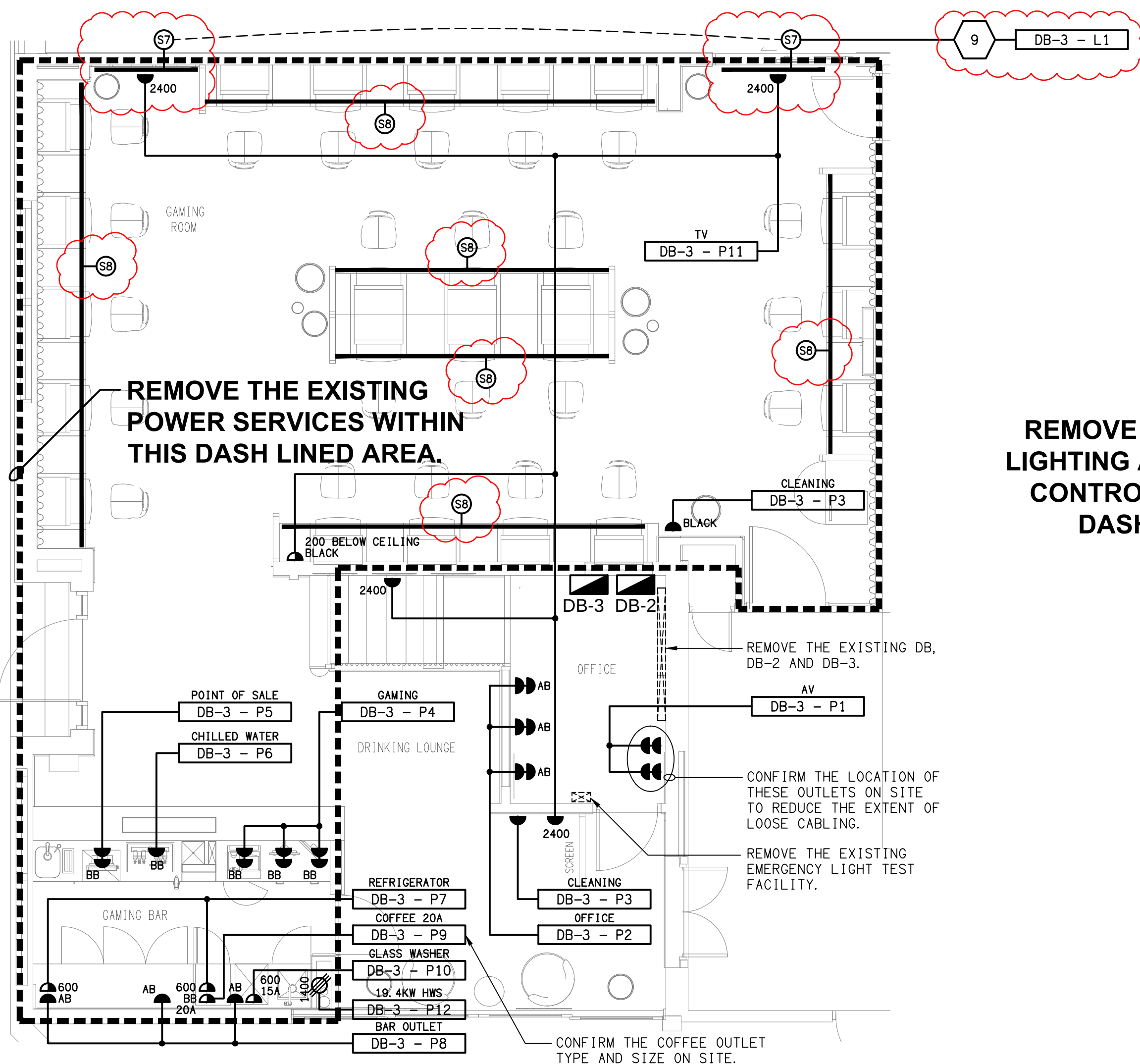
FLOOR PLAN GAMING ROOM REFURBISHMENT SCALE 1:50
