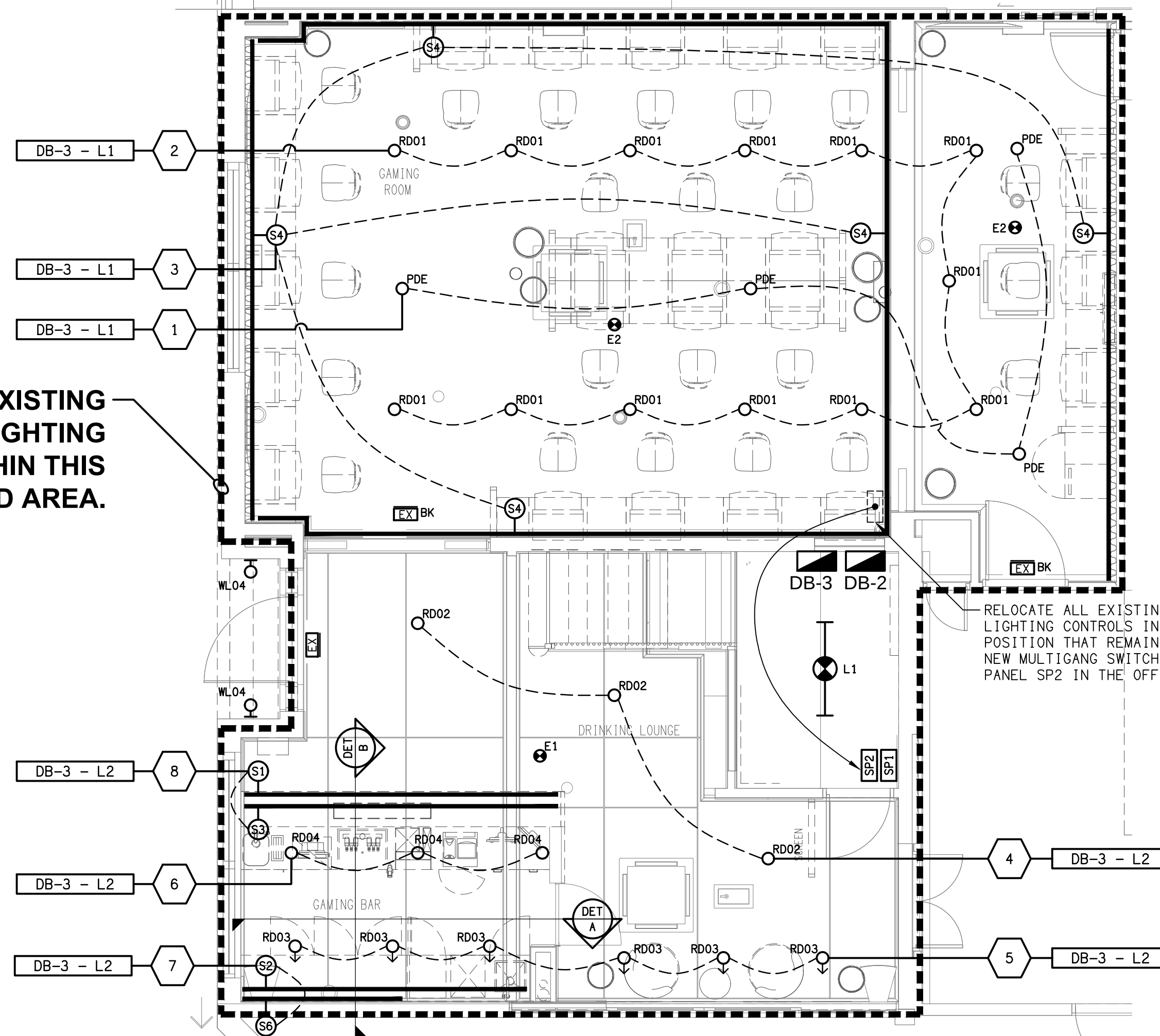
REFLECTED CEILING PLAN GAMING ROOM REFURBISHMENT SCALE 1:50
