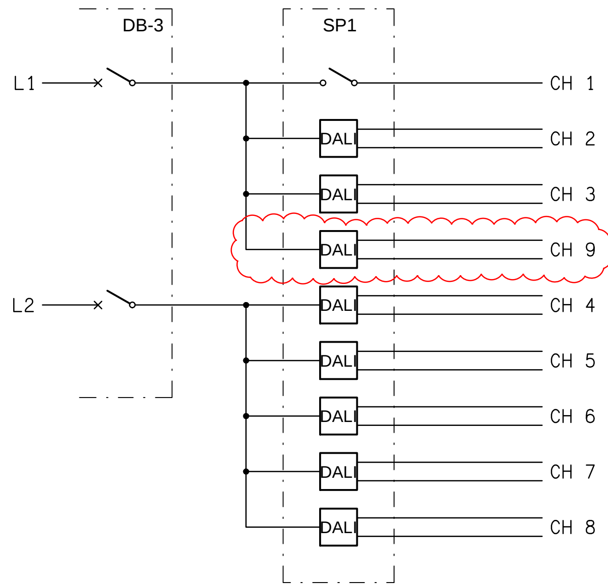
SCHEMATIC LIGHTING CONTROL SP1 NOT TO SCALE
